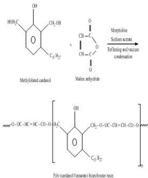
Reaction Scheme 1: Synthesis of Poly (Cardanol Fumarate) Biopolyester Resin
