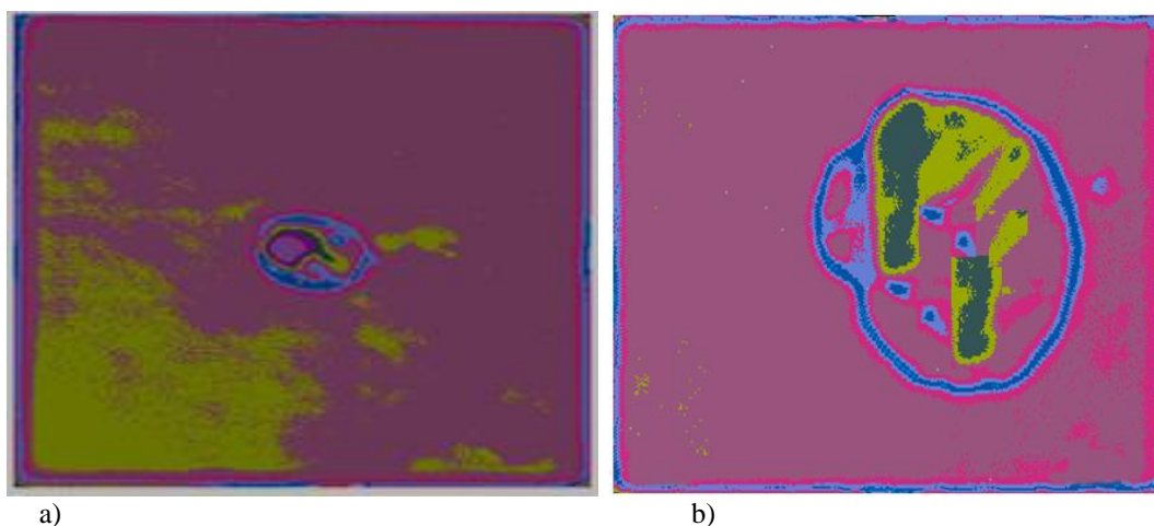
Figure 8: C-scan image of a 30J and 50J impacts using the round impactor [1], [10]
