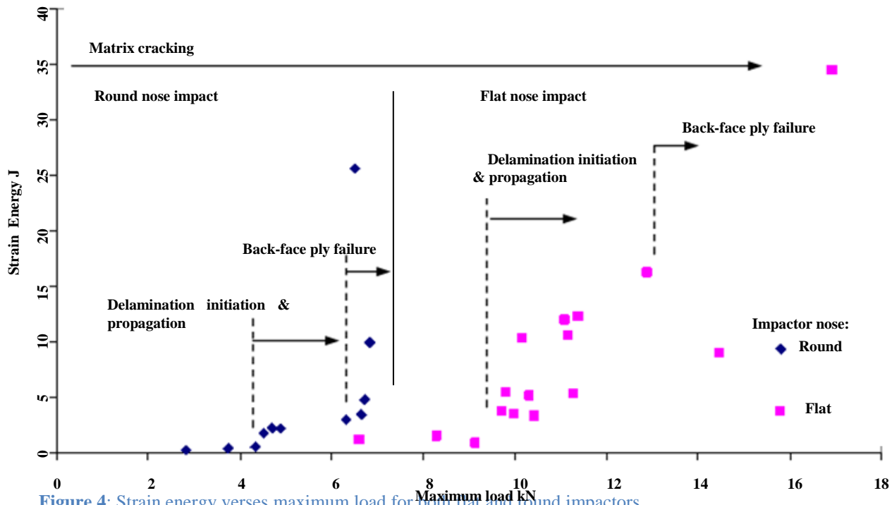
Figure 4: Strain energy versus maximum load for both flat and round impactors.
