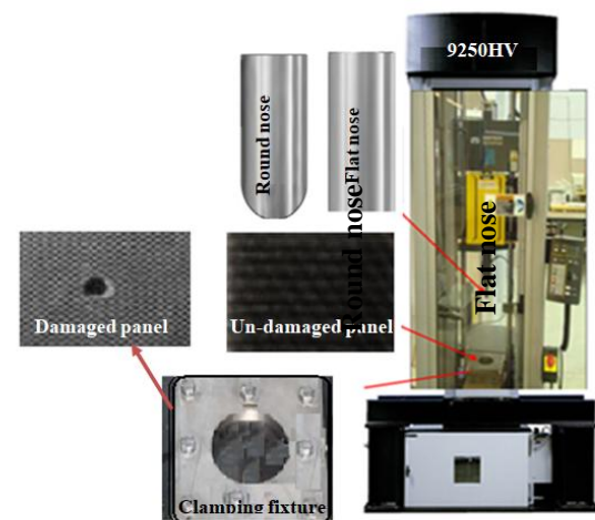
Figure 2: Schematic of INSTRON™ 9250HV impact test machine
