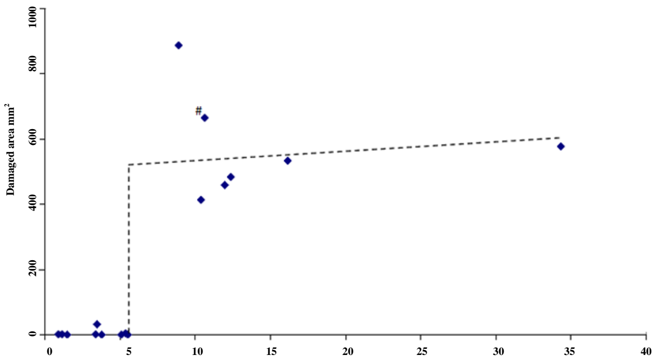
Figure 11: Damage area verses strain energy for the flat impactor.
