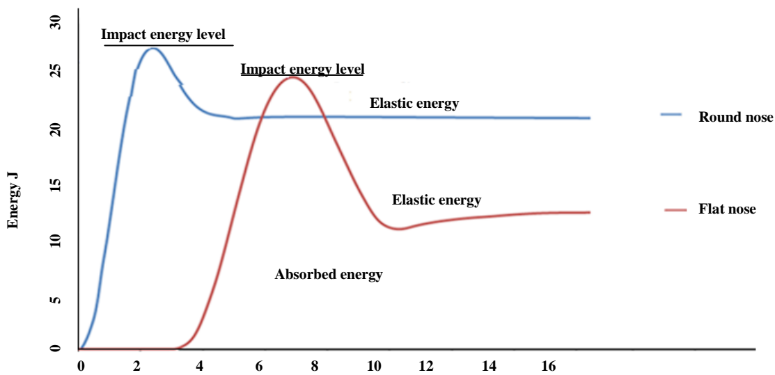
Figure 13: Energy-histories of 16-Ply laminate at velocity 3.12 m/s
