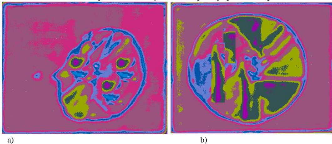
Figure 9: C-scan image of 30J and 50J impacts using the flat impactor [1], [10]
