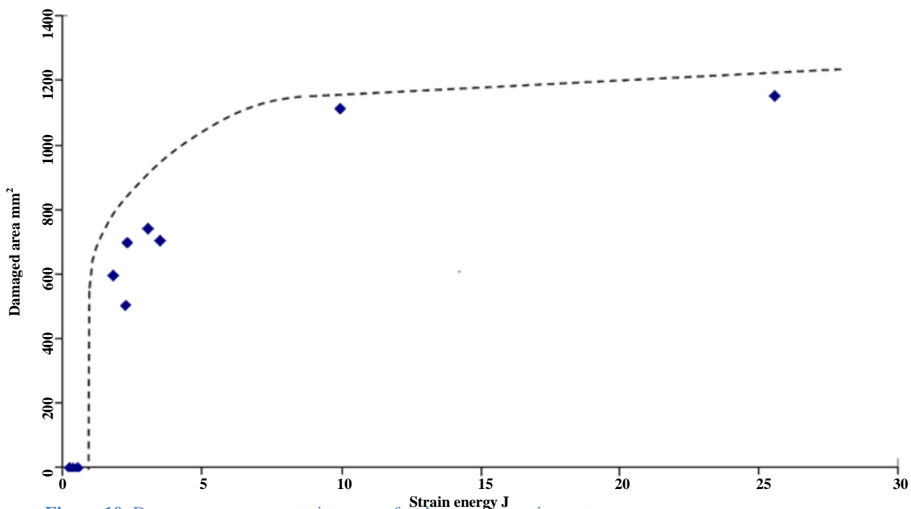
Figure 10: Damage area versus strain energy for the round nose impactor.
